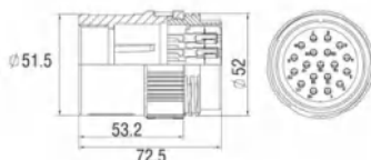
19-PIN MALE PLUG 19芯公插
