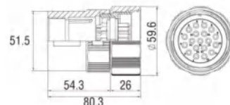
19-PIN FEMALE PLUG 19芯母插
