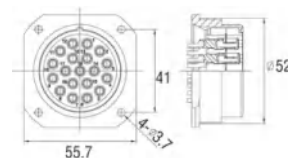
19-PIN MALE SOCKET 19芯公座
